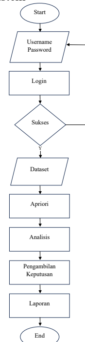
Gambar 2. Flowchart Sistem
