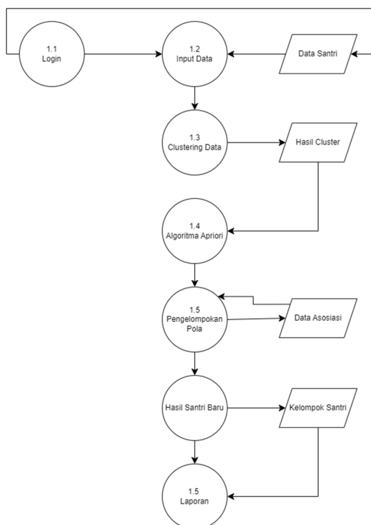
Gambar 4. DFD Level 1
