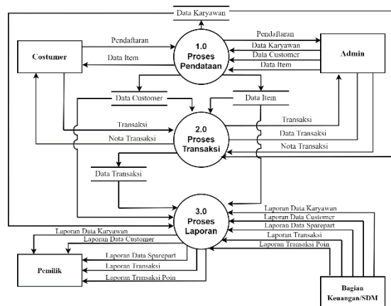
Gambar 3. Diagram Nol
